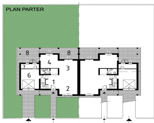
PLAN PARTER
